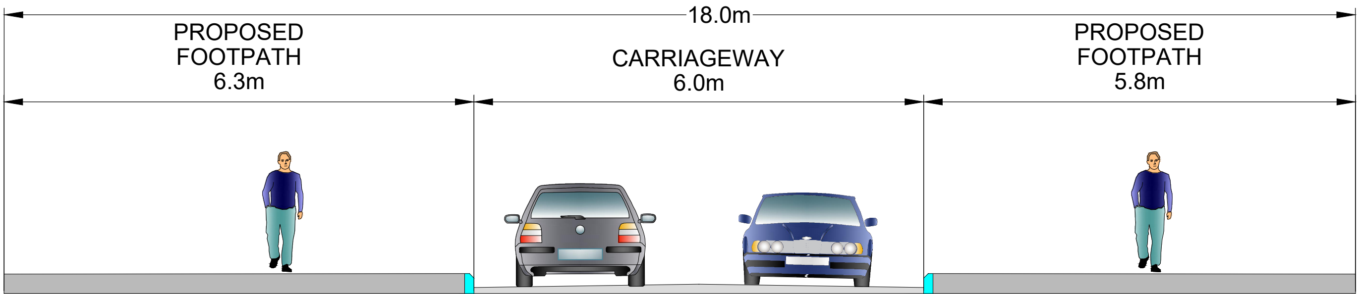
CROSS SECTION K-K
